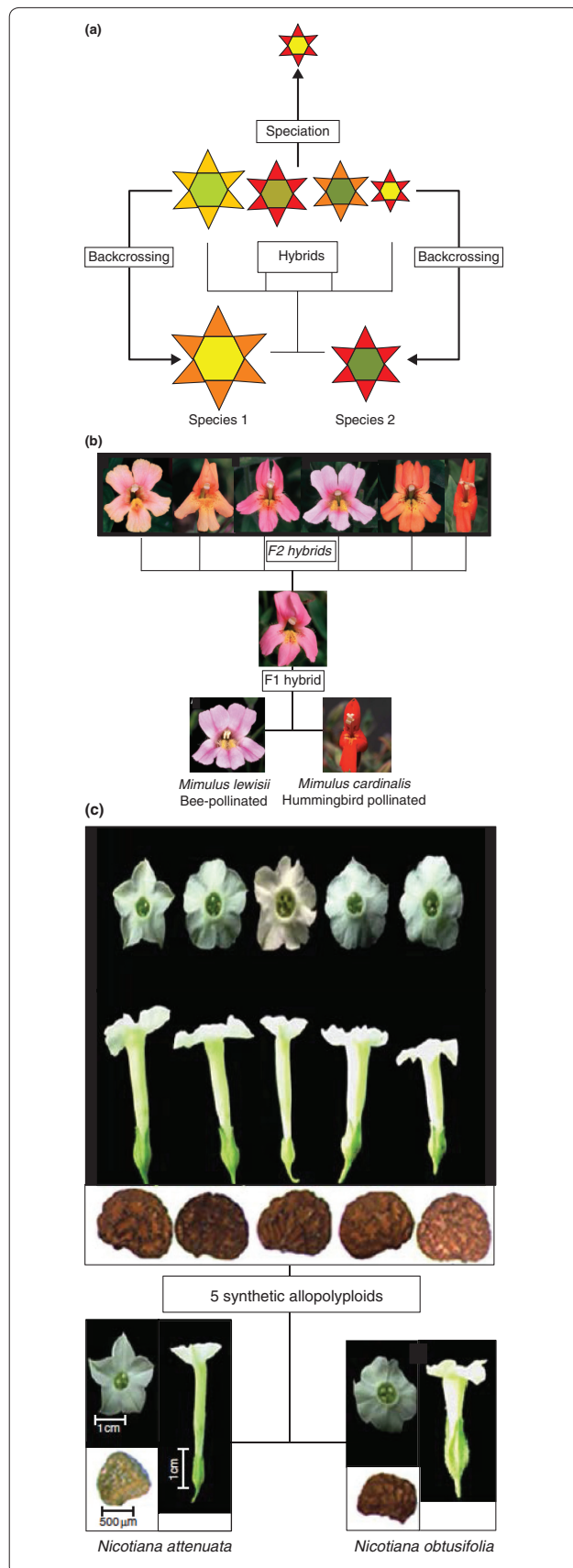
Figure 2. Hybridization, polyploidy and flower phenotypes.
